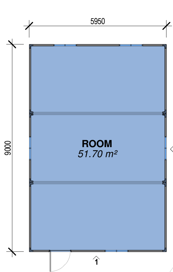
FLOOR PLAN
