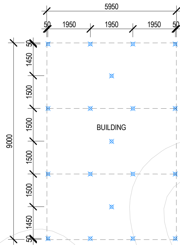
SUPPORT PLAN
