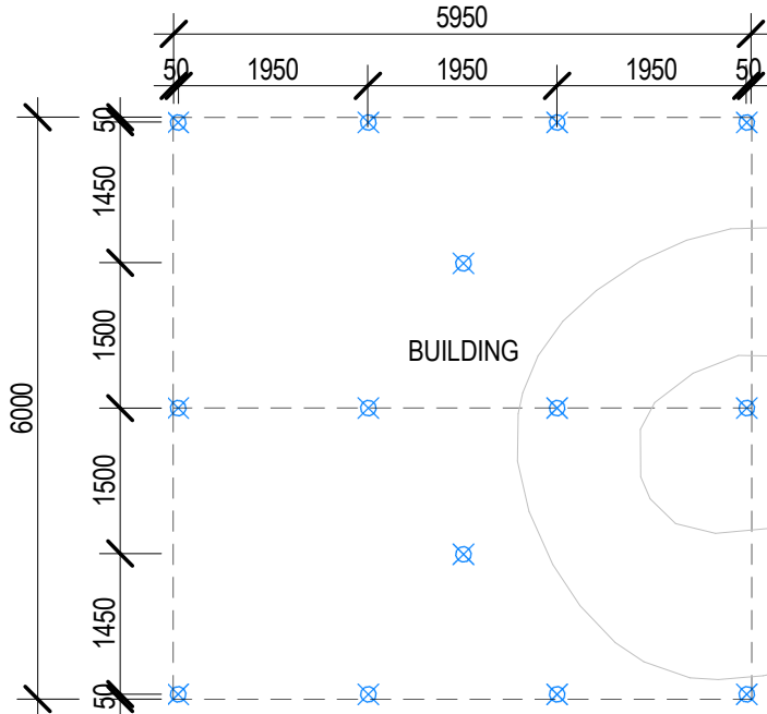
SUPPORT PLAN
