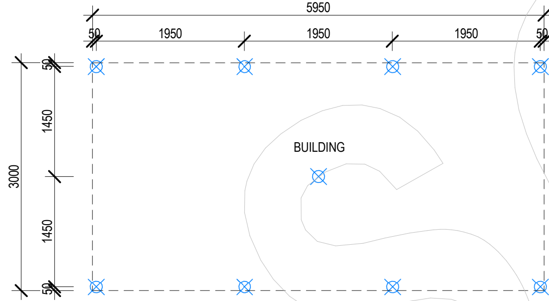
FLOOR PLAN
