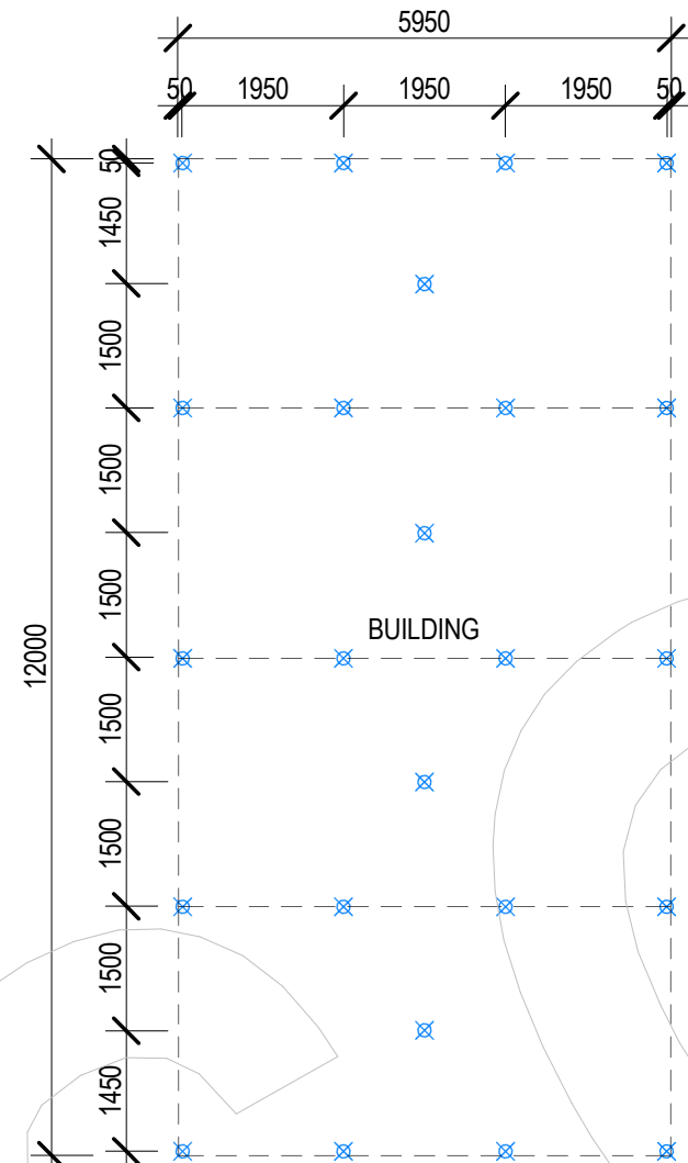
SUPPORT PLAN
